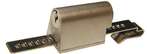
722S-26D Plunger lock For Best style, small format IC core
