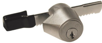
N078-26D78 Diamond back desk/cabinet lock National keyway
