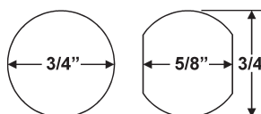
MOUNTING CUTOUT
