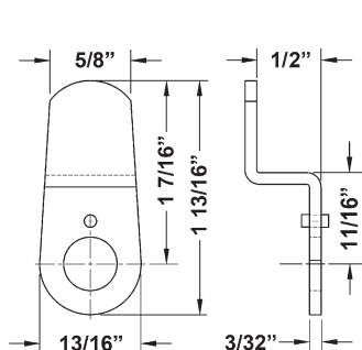
DCNP-100-HD 1-7/16" long cam, 1/2" offset
