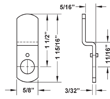
DCNP-100-LBC 1-1/2" long cam, 5/16" offset
