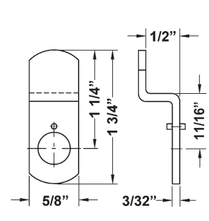
DCNP-100-BC5 1-1/4" long cam, 1/2" offset
