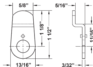
DCNP-100-HD3 1-1/8" long cam, 5/16" offset
