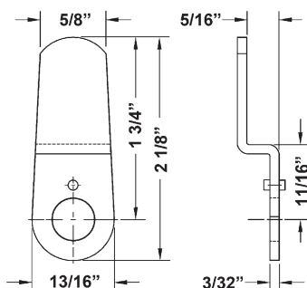
DCNP-100-HD2 1-3/4" long cam, 5/16" offset
