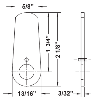
DCNP-100-SC2 1-3/4" heavy duty straight cam
