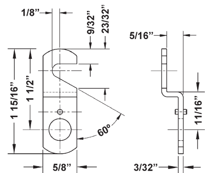
DCNP-100-HC1 1-1/2" long hook cam, 5/16" offset
