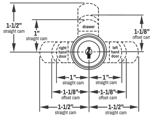
Dimensional offset of 1-1/8" cam is 11/32"
